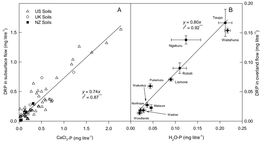
Figure X Relationship between DRP in subsurface flow and \text{CaCl}_2\text{-P} for US (McDowell & Sharpley 2001), UK (McDowell & Sharpley 2001) and NZ (McDowell & Monaghan 2002; McDowell unpublished) soils (A), and between DRP in overland flow and \text{H}_2\text{O-P} for selected New Zealand grassland soils (B). Error bars are the standard errors for 3 replicates.
