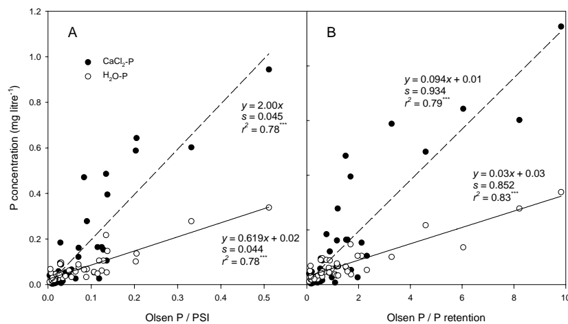
Figure X Linear regressions for the relationships between DRP concentration in \text{CaCl}_2\text{-P} or \text{H}_2\text{O-P} and the quotients of Olsen P and PSI (A), and Olsen P and % P retention (B) for 44 New Zealand grassland soils.
